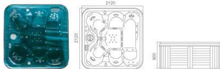
1. MODEL:WS-092B SIZE:2120X2120X900mm
