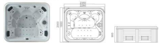
2. MODEL:WS-093A SIZE:2350X2000X900mm
